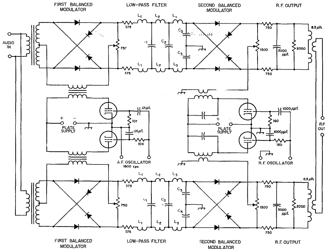
Fig. 1 — Circuit of the "third method" single-side-band generator (Weaver, Proc. IRE , December, 1956). Constants of output circuits of second balanced modulators (3000 \mu\mu\text{f.} and 8.5 \mu\text{h.} ) and the RC values in the r. f. oscillator phase-shift network (160 ohms and 1000 \mu\mu\text{f.} ) are for an output frequency of 1 Mc. and should be modified appropriately for other output frequencies. Low-pass filter constants are as follows:
